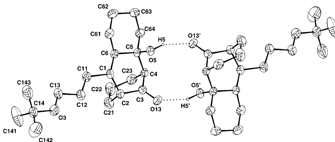
Figure 3. View of two enantiomers of 4 linked by hydrogen bonds with atom labelling scheme; ellipsoids are drawn at 30% probability
