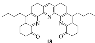
Figure 4. Annelated polypyridine for the selective complexation of sodium and potassium
