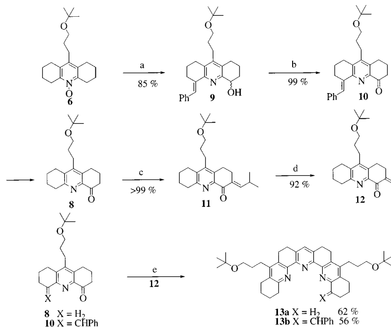
Scheme 2. (a) Ac 2 O/PhCHO 2:1, 170 °C; saponification with 2 M K 2 CO 3 solution; (b) DMSO, oxalyl chloride, CH 2 Cl 2 , Et 3 N, -78 °C; (c) tert -butoxybis(dimethylaminomethane), 45 °C, 3 h; (d) diisobutylaluminium hydride, THF, -78 °C, 2 h, NH 4 Cl; (e) pyridine, NH 4 OAc, 90 °C
