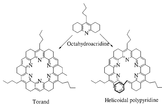
Figure 1. Synthesis of soluble annelated polypyridines from 9-butyloctahydroacridine
