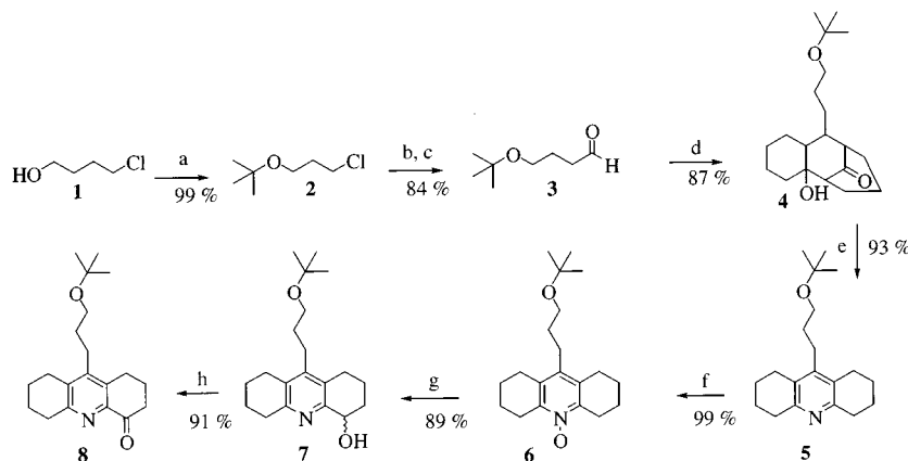
Scheme 1. (a) Isobutene, \text{H}_2\text{SO}_4 (cat.), \text{CH}_2\text{Cl}_2 , -78^\circ\text{C} ; (b) Mg, (\text{CH}_2)_2\text{Br}_2 , THF, reflux; (c) N -formylpiperidine, THF, -20^\circ\text{C} , 3 N HCl; (d) cyclohexanone, EtONa/EtOH, reflux; (e) AcOH, \text{Cu}(\text{OAc})_2 , \text{NH}_4\text{OAc} ; (f) m -chloroperbenzoic acid, \text{CH}_2\text{Cl}_2 , 0^\circ\text{C} ; (g) trifluoroacetic anhydride, \text{CH}_2\text{Cl}_2 , room temp.; saponification with 2 M \text{K}_2\text{CO}_3 solution; (h) DMSO, oxalyl chloride, \text{CH}_2\text{Cl}_2 , \text{Et}_3\text{N} , -78^\circ\text{C}
