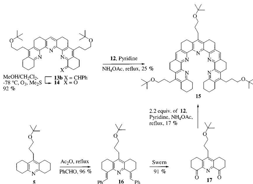
Scheme 3. Synthesis of the annulated quinqueterpyridine 15 with 11 adjacent rings
