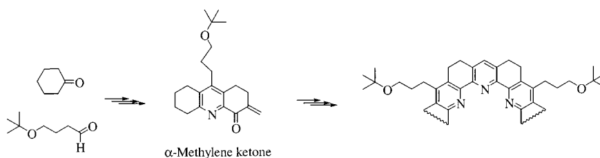
Figure 2. Synthetic strategy for the new annelated polypyridines
